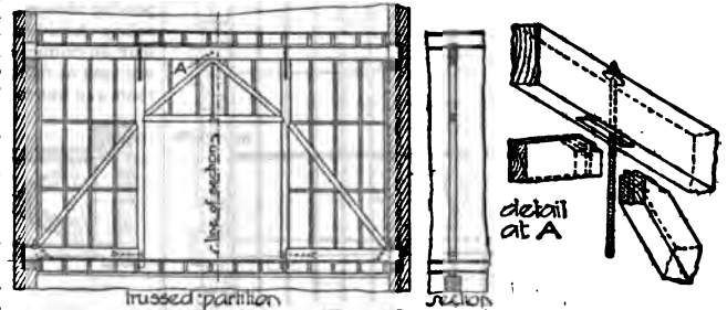
FIG. 31.—Trussed Partition.
