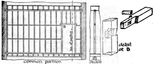
FIG. 30.—Common Partition.
