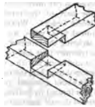
FIG. 11.—Bevelled Halving.
