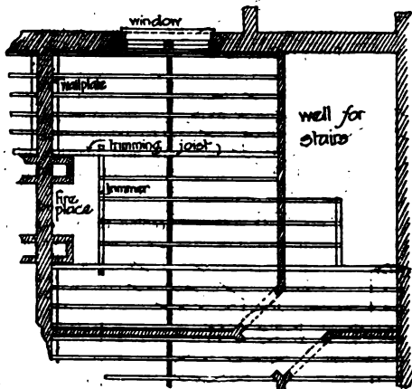
FIG. 23.—Single Floor.
