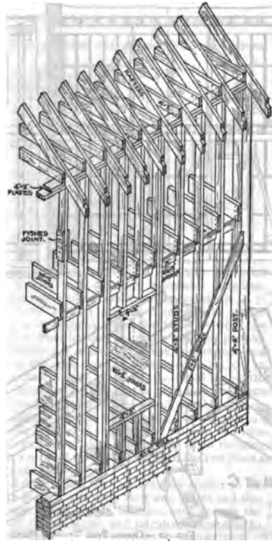
FIG. 36.—Balloon Frame.
