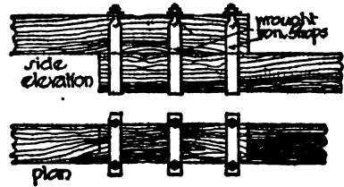
FIG. 1.—Lapped Joint.
