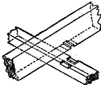
FIG. 7.—Cogging.
