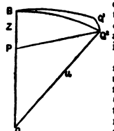
FIG. 2. The section whose radius of curvature is R_1 . Then if O is the centre of curvature in the plane of the paper, and BO = u ,
