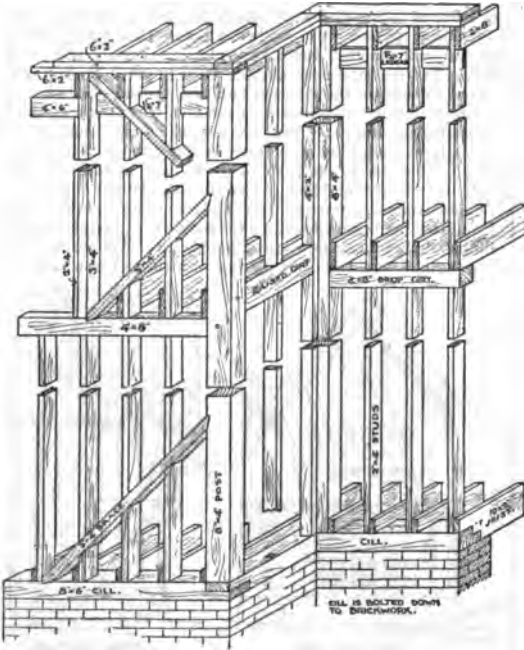
FIG. 35.—Braced Frame.
