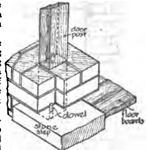
FIG. 19.—Dowelling.
