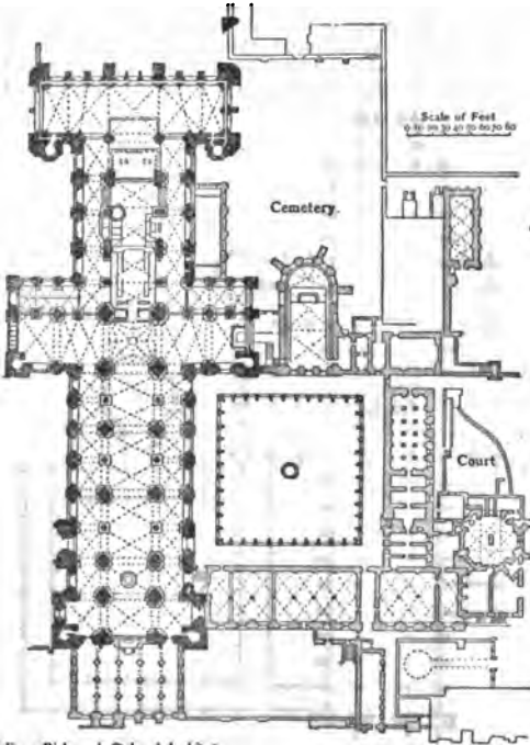
FIG. 3.—Plan of Durham Cathedral.
