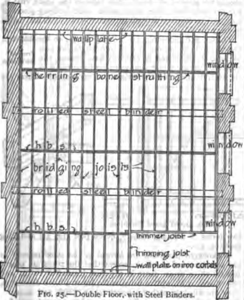
FIG. 25.—Double Floor, with Steel Binders.
