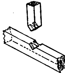
FIG. 17.—Bridle Joint.
