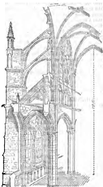
FIG. 8.—Perspective of Amiens Cathedral.
