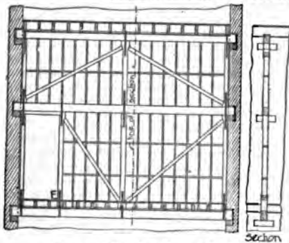
FIG. 33.—King Post Trussed Partition.
