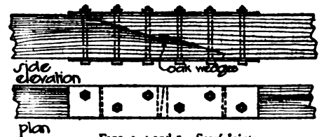
FIGS. 3, 4 and 5.—Scarf Joints.
