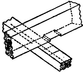
FIG. 6.—Notching.
