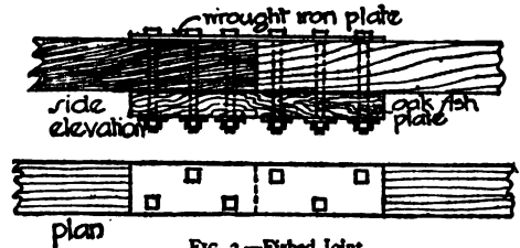
FIG. 2.—Fished Joint.
